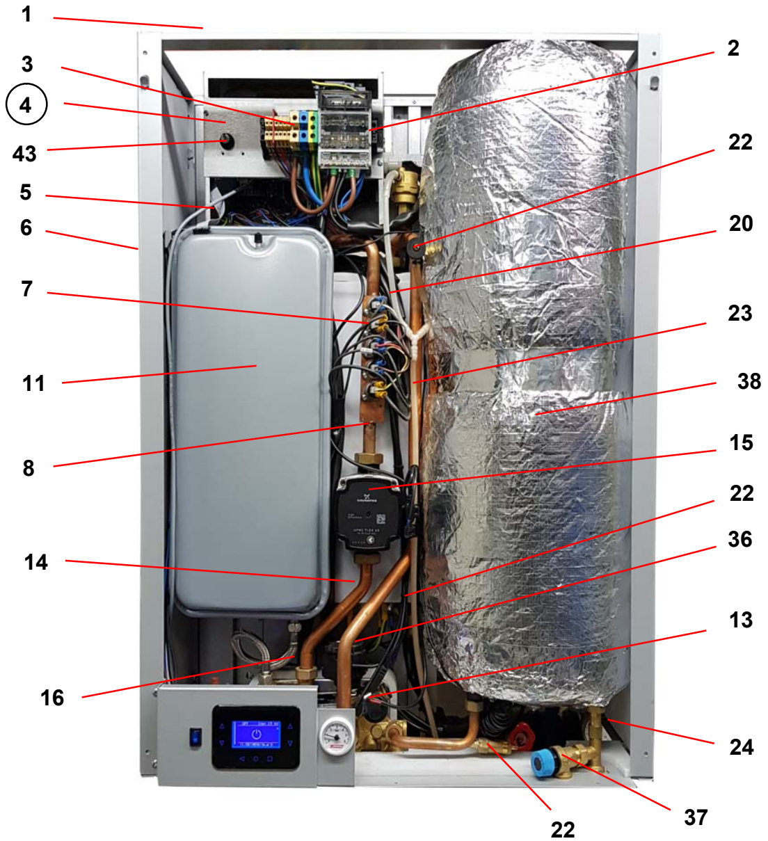
4 Detail view: Electric Box
