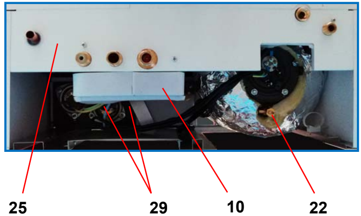
Detail view: Body / Heating Elements
